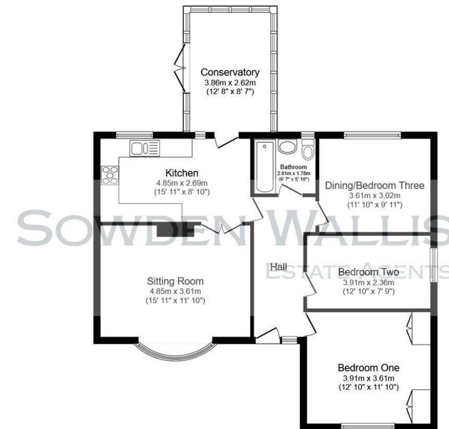
Floor Plan
